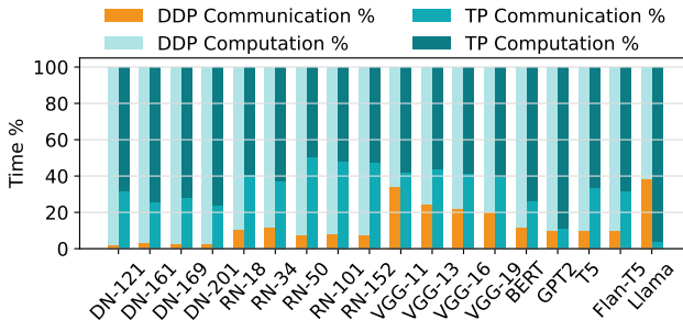
Figure 13: Communication and computation time ratio for models training with tensor parallelism and distributed data parallelism simulations on P1.
